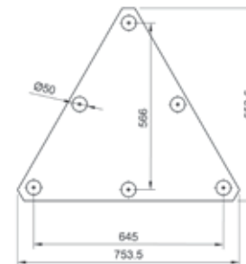
Base mounting locations & wiring diagram M8 Thread
