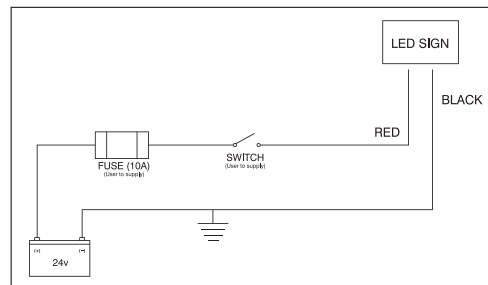
Base mounting locations & wiring diagram M8 Thread
