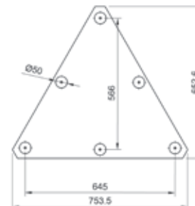
Base mounting locations & wiring diagram M8 Thread
